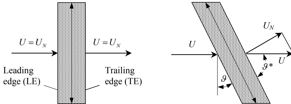
Fig 2: Angles and velocities for unswept and swept blades
