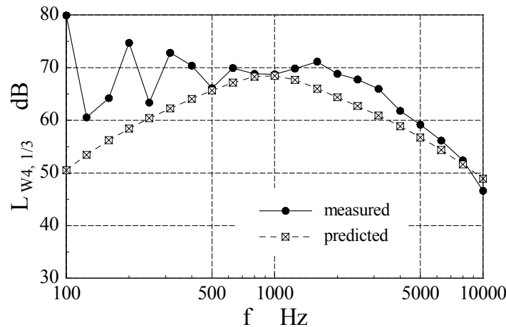
Fig. 1: Computed ([10]) and measured noise spectrum of an axial fan
