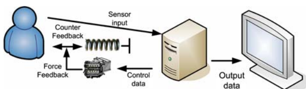
Fig. 7 A hybrid counter and force feedback architecture for the Exertion Interface
