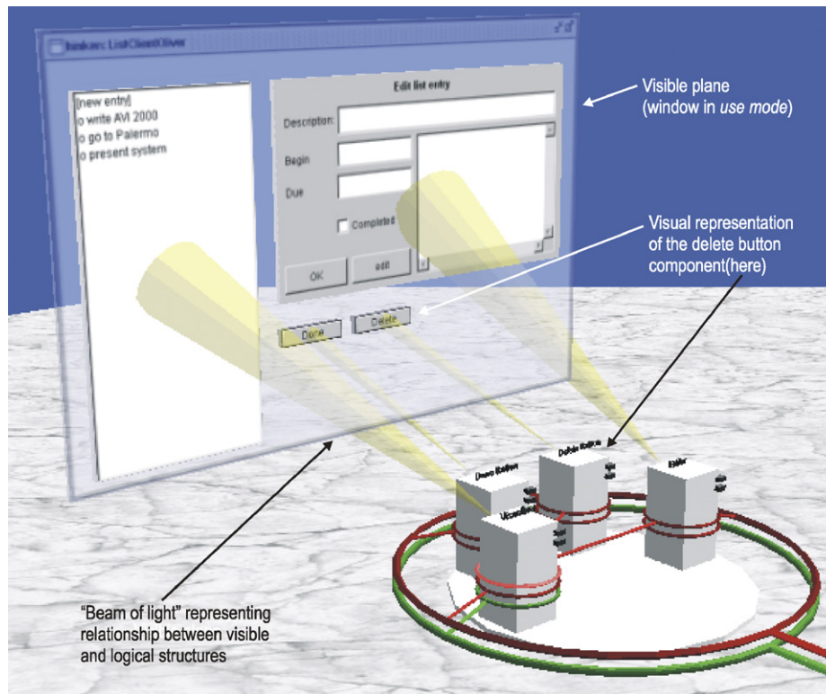
Fig. 4. 3D graphical tailoring interface displaying a client's tailorable component structure.
