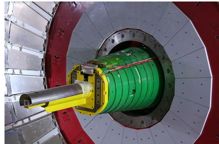
CMS-Experiment im Large Hadron Collider
